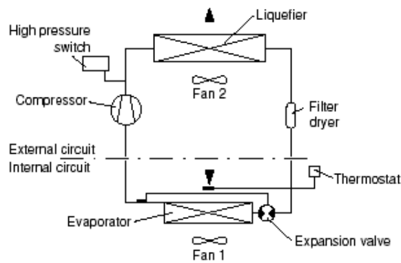
Fig. 8.1 Cooling Circuit
