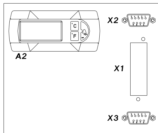
Fig. 6.2 Control panel / connector panel
